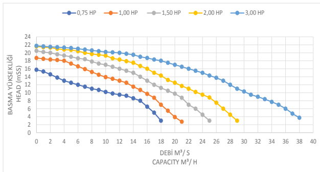
Performance Curves
