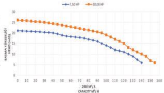
Performance Curves
